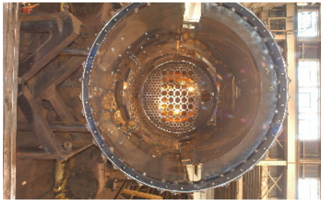
Flue Sheets
